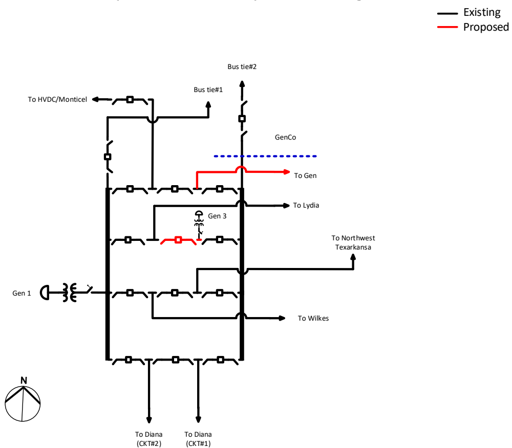
Figure 1: Point of Interconnection (POI INFORMATION) One-Line Diagram
